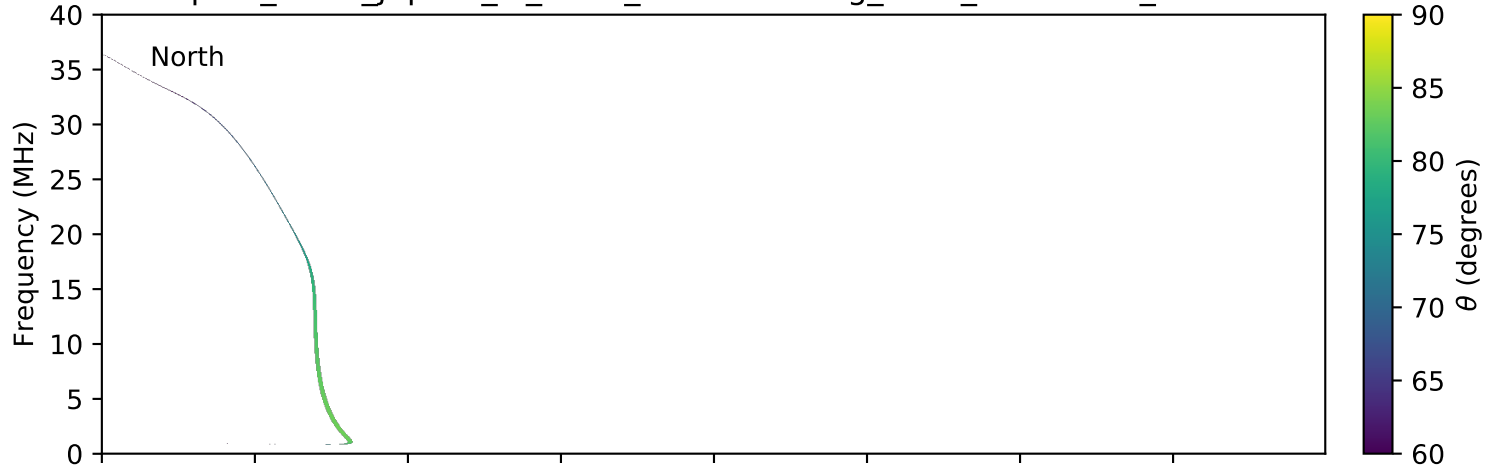
expres_earth_jupiter_io_isaac_lossc-wid1deg_3kev_20080223_v01.cdf
