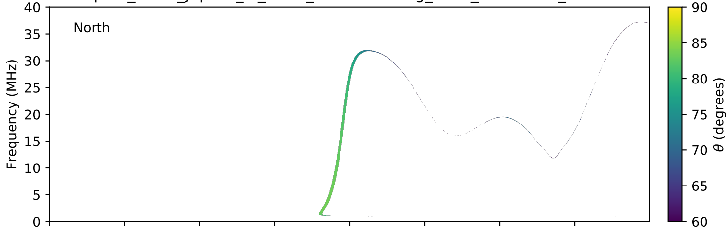
expres_earth_jupiter_io_isaac_lossc-wid1deg_3kev_20080222_v01.cdf
