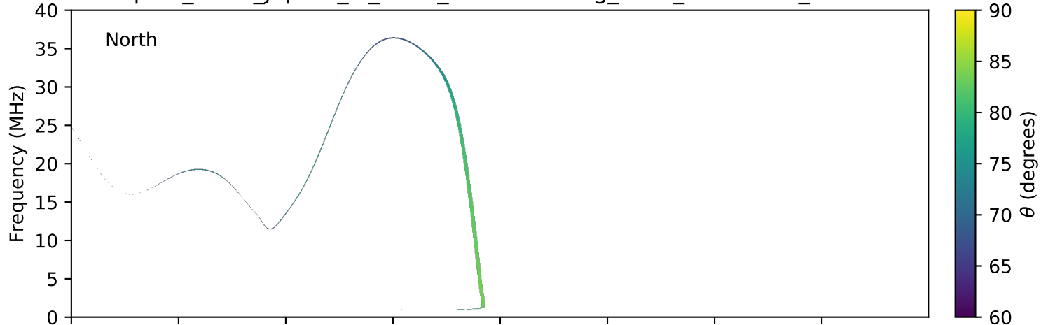
expres_earth_jupiter_io_isaac_lossc-wid1deg_3kev_20080221_v01.cdf
