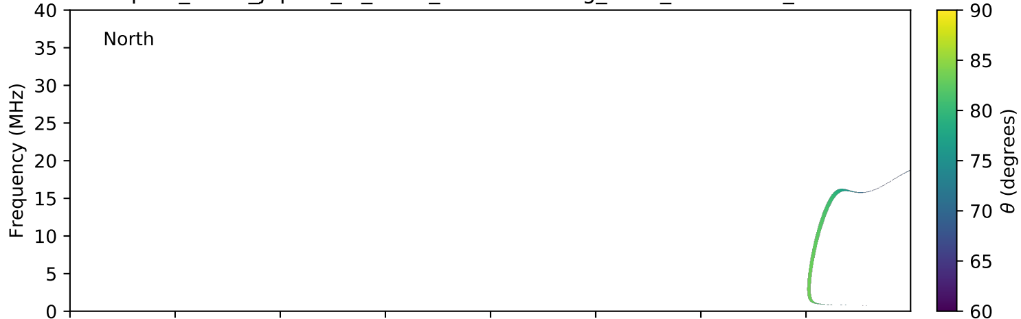
expres_earth_jupiter_io_isaac_lossc-wid1deg_3kev_20080218_v01.cdf
