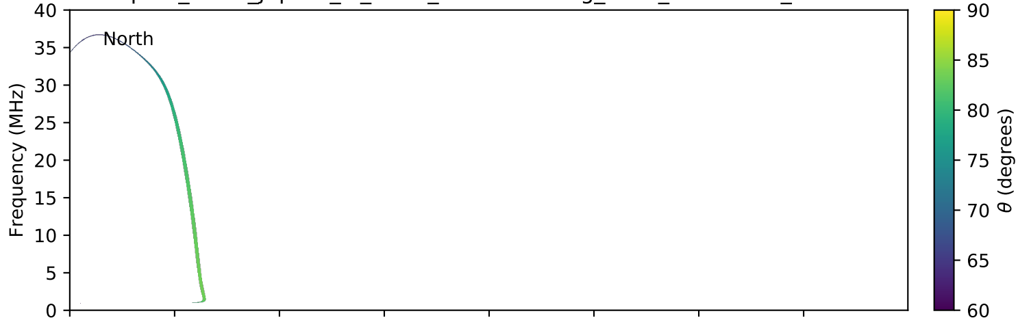
expres_earth_jupiter_io_isaac_lossc-wid1deg_3kev_20080216_v01.cdf
