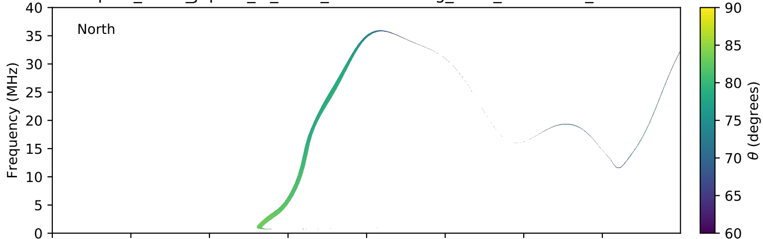
expres_earth_jupiter_io_isaac_lossc-wid1deg_3kev_20080215_v01.cdf
