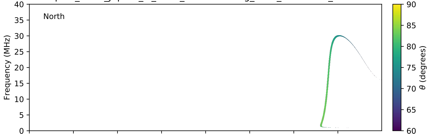
expres_earth_jupiter_io_isaac_lossc-wid1deg_3kev_20080211_v01.cdf
