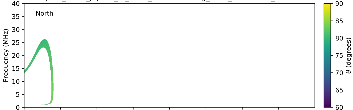
expres_earth_jupiter_io_isaac_lossc-wid1deg_3kev_20080209_v01.cdf
