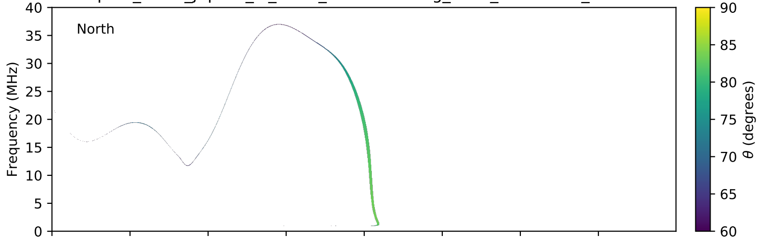
expres_earth_jupiter_io_isaac_lossc-wid1deg_3kev_20080205_v01.cdf
