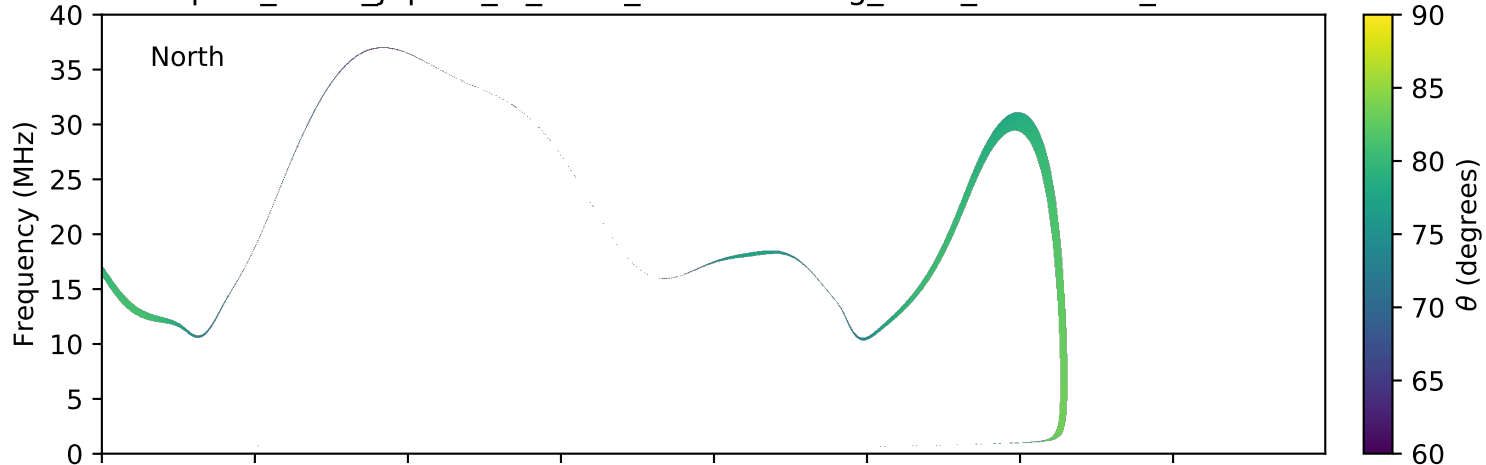
expres_earth_jupiter_io_isaac_lossc-wid1deg_3kev_20080203_v01.cdf
