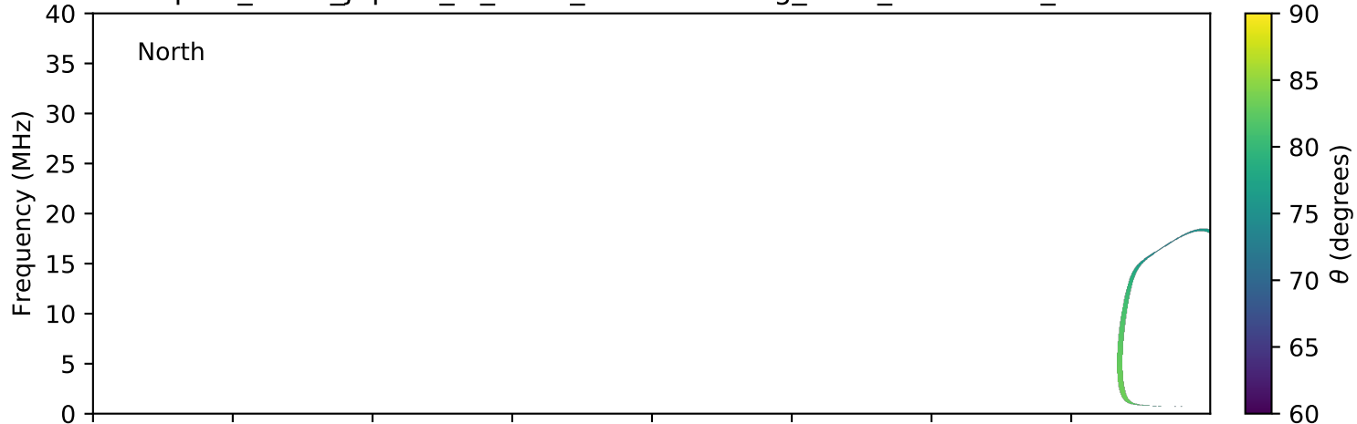
expres_earth_jupiter_io_isaac_lossc-wid1deg_3kev_20080202_v01.cdf
