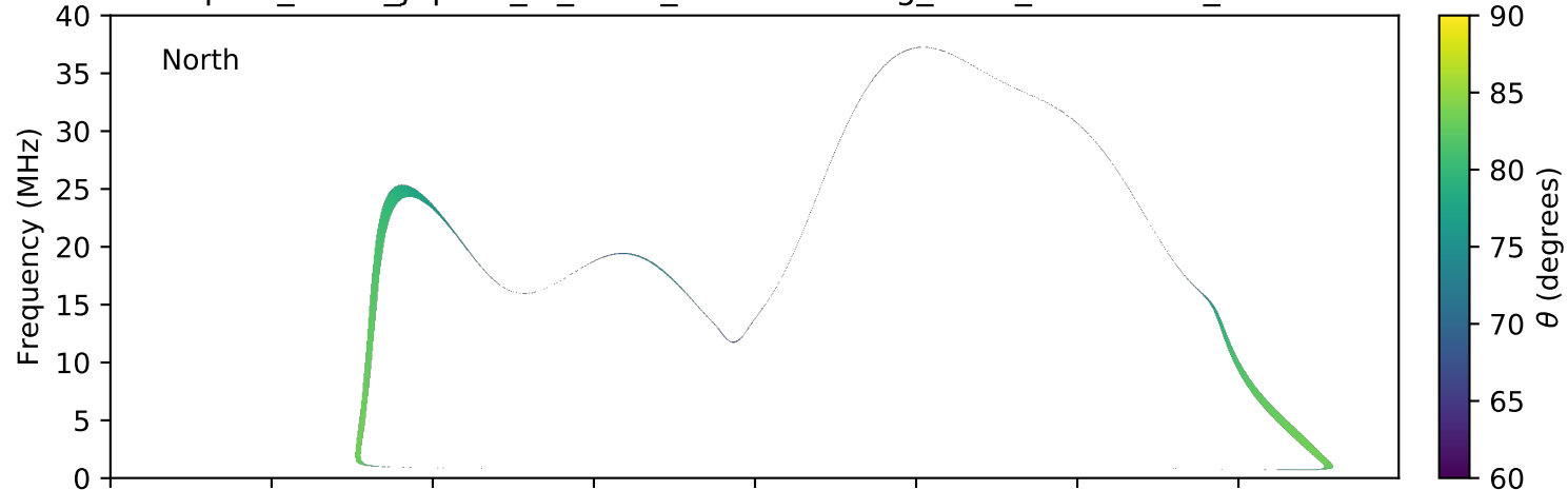
expres_earth_jupiter_io_isaac_lossc-wid1deg_3kev_20080201_v01.cdf
