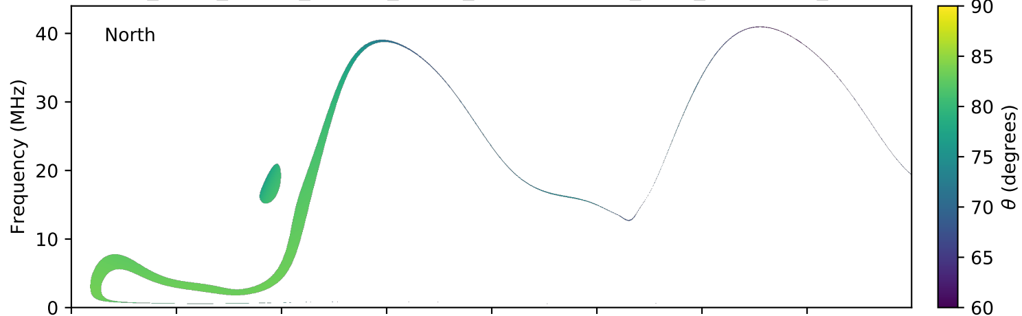
expres_earth_jupiter_europa_jrm09_lossc-wid1deg_3kev_20080226_v01.cdf
