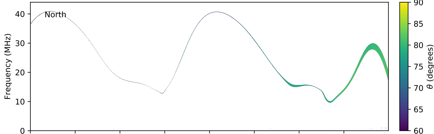
expres_earth_jupiter_europa_jrm09_lossc-wid1deg_3kev_20080216_v01.cdf
