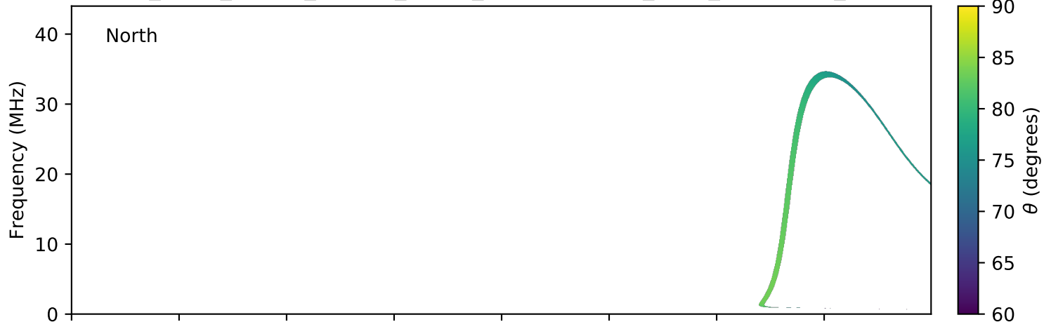
expres_earth_jupiter_europa_jrm09_lossc-wid1deg_3kev_20080204_v01.cdf
