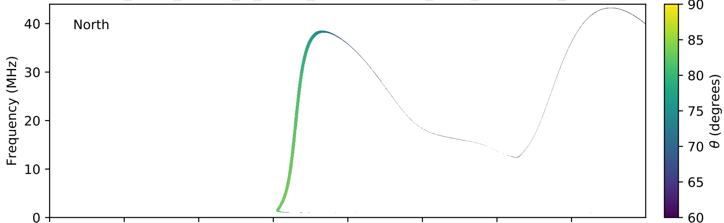
expres_earth_jupiter_io_jrm09_lossc-wid1deg_3kev_20080123_v01.cdf
