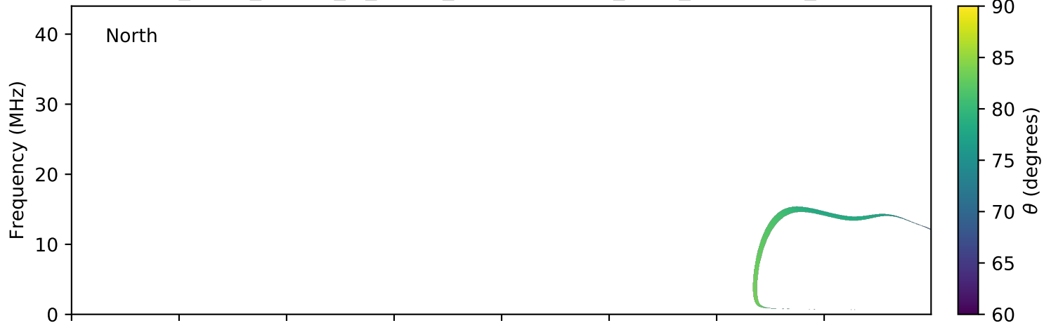
expres_earth_jupiter_io_jrm09_lossc-wid1deg_3kev_20080119_v01.cdf
