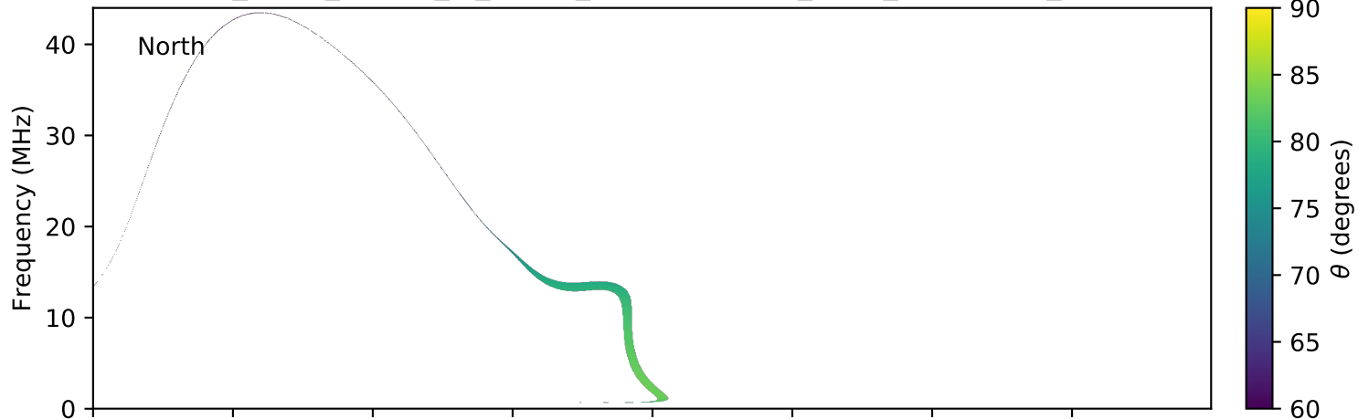
expres_earth_jupiter_io_jrm09_lossc-wid1deg_3kev_20080113_v01.cdf
