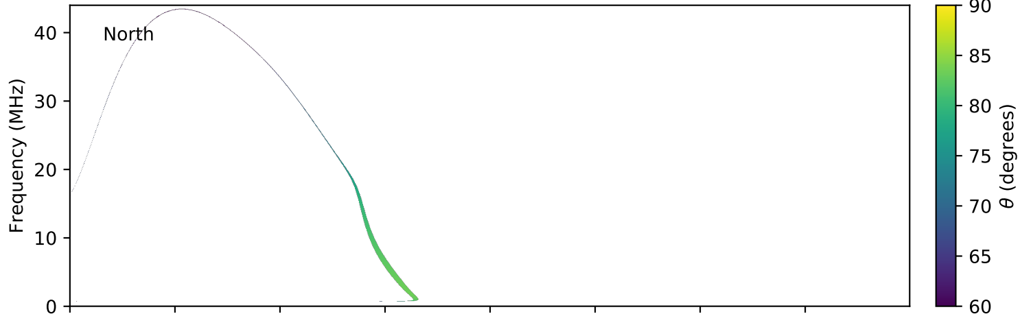
expres_earth_jupiter_io_jrm09_lossc-wid1deg_3kev_20080106_v01.cdf
