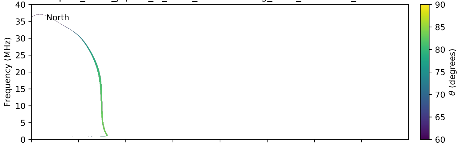
expres_earth_jupiter_io_isaac_lossc-wid1deg_3kev_20080131_v01.cdf
