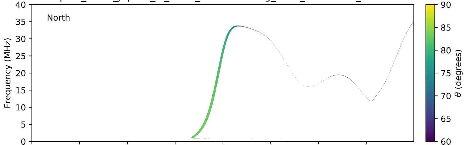
expres_earth_jupiter_io_isaac_lossc-wid1deg_3kev_20080130_v01.cdf
