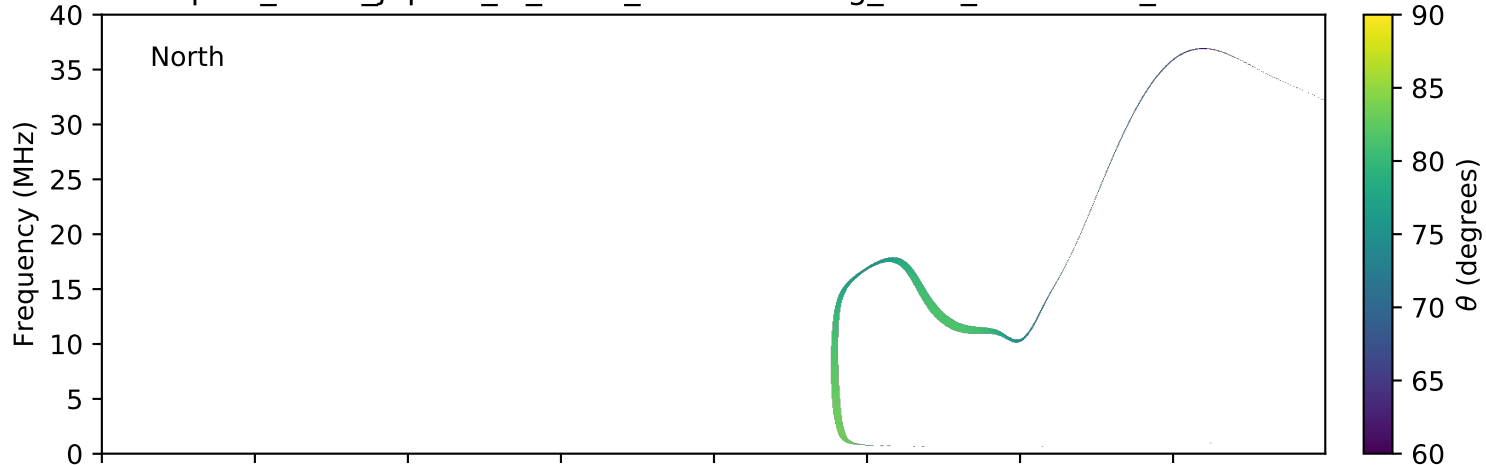
expres_earth_jupiter_io_isaac_lossc-wid1deg_3kev_20080128_v01.cdf
