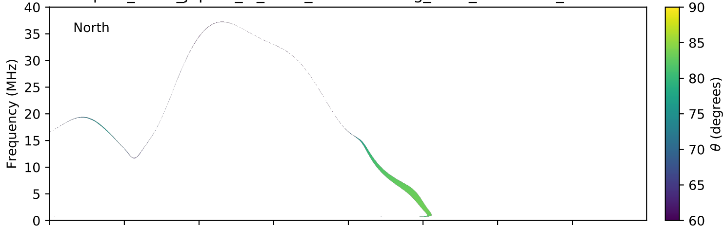
expres_earth_jupiter_io_isaac_lossc-wid1deg_3kev_20080127_v01.cdf
