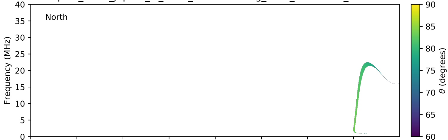
expres_earth_jupiter_io_isaac_lossc-wid1deg_3kev_20080126_v01.cdf
