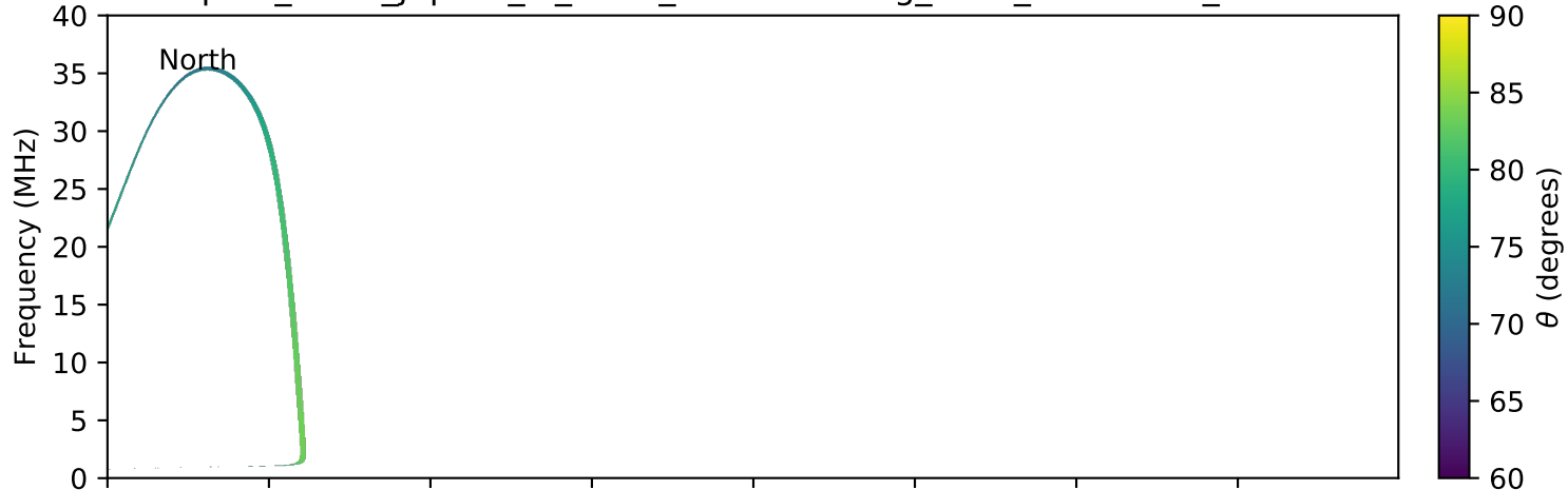
expres_earth_jupiter_io_isaac_lossc-wid1deg_3kev_20080124_v01.cdf
