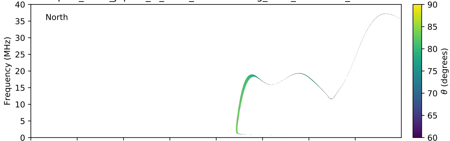
expres_earth_jupiter_io_isaac_lossc-wid1deg_3kev_20080121_v01.cdf
