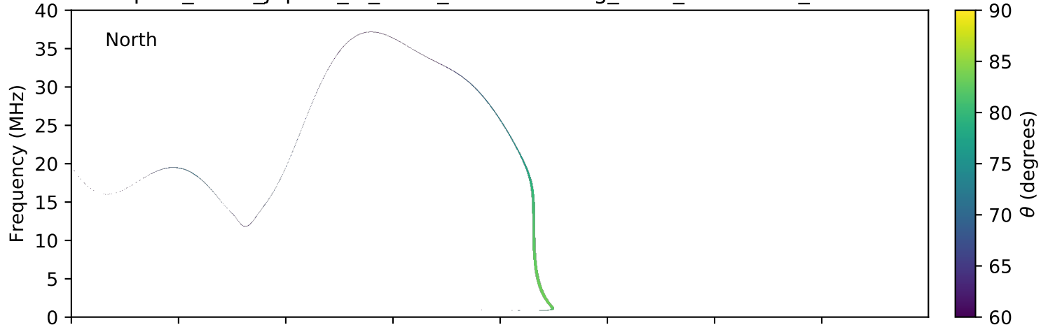
expres_earth_jupiter_io_isaac_lossc-wid1deg_3kev_20080120_v01.cdf
