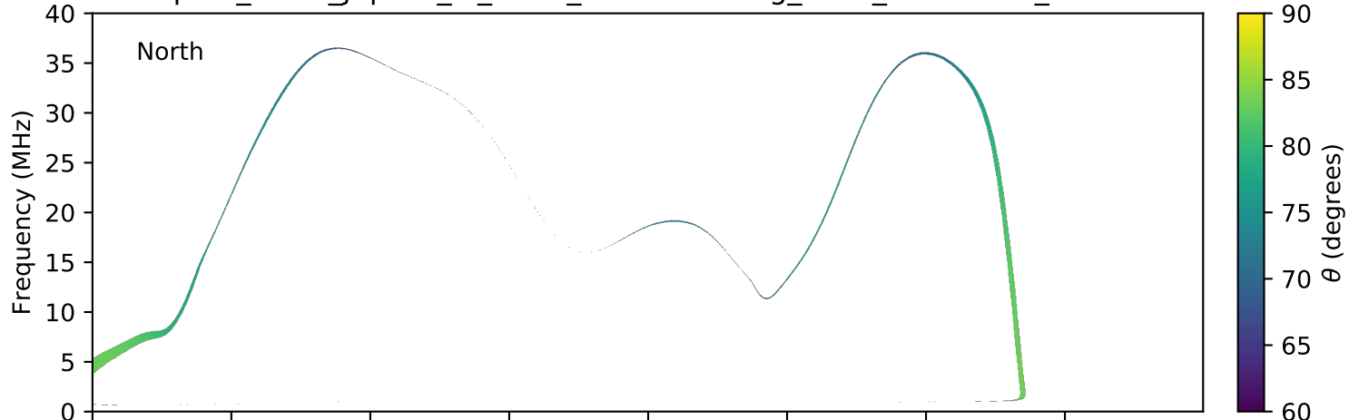
expres_earth_jupiter_io_isaac_lossc-wid1deg_3kev_20080118_v01.cdf
