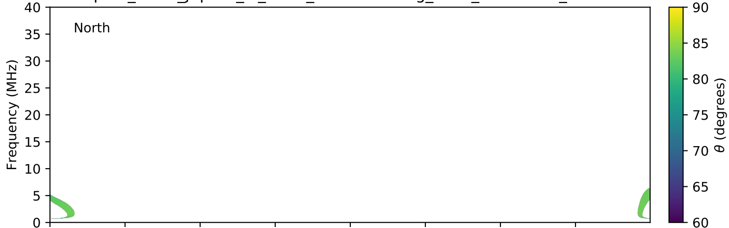
expres_earth_jupiter_io_isaac_lossc-wid1deg_3kev_20080117_v01.cdf
