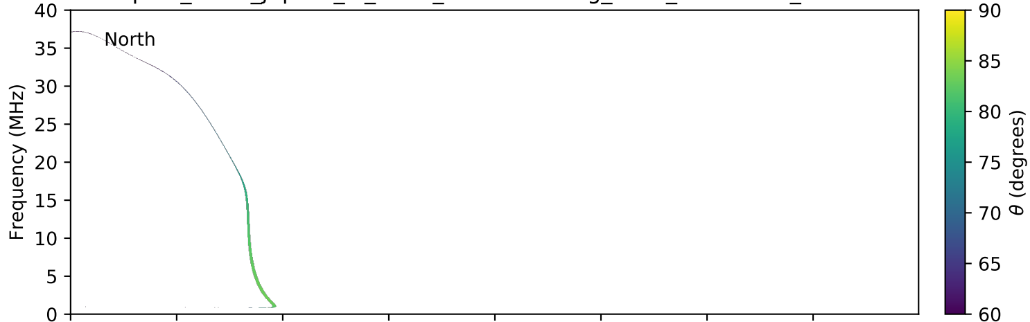
expres_earth_jupiter_io_isaac_lossc-wid1deg_3kev_20080115_v01.cdf
