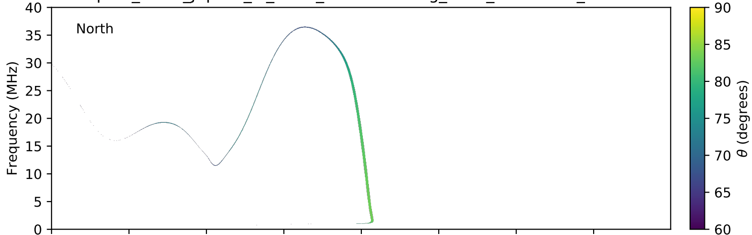
expres_earth_jupiter_io_isaac_lossc-wid1deg_3kev_20080113_v01.cdf
