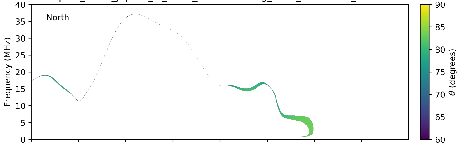
expres_earth_jupiter_io_isaac_lossc-wid1deg_3kev_20080111_v01.cdf
