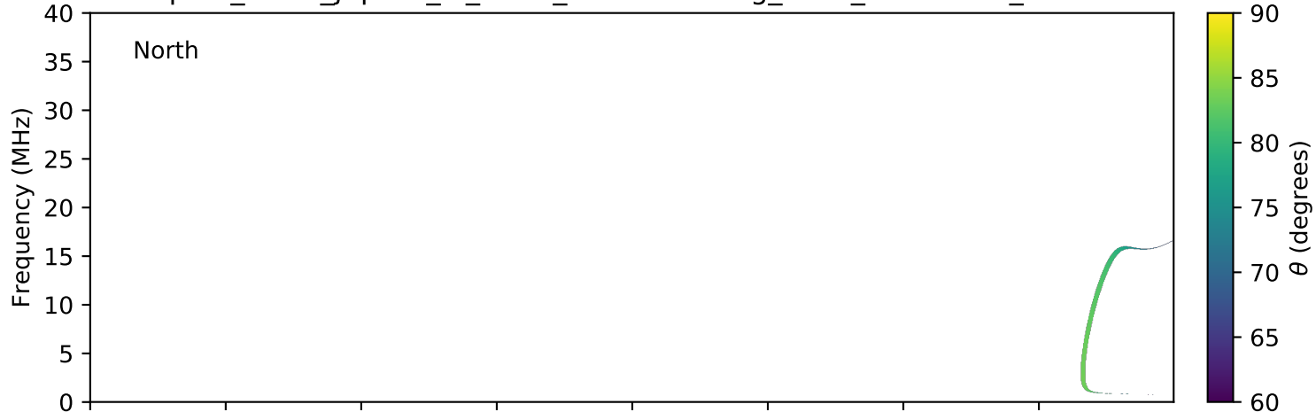
expres_earth_jupiter_io_isaac_lossc-wid1deg_3kev_20080110_v01.cdf
