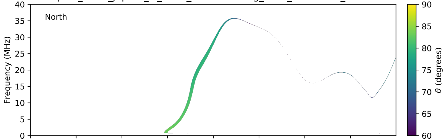
expres_earth_jupiter_io_isaac_lossc-wid1deg_3kev_20080107_v01.cdf
