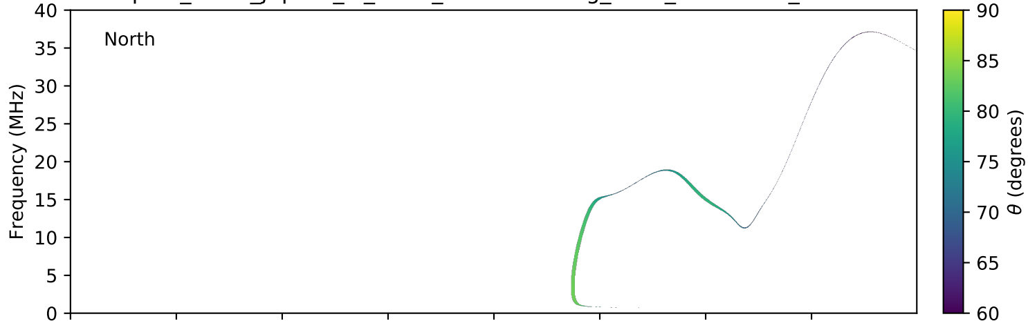
expres_earth_jupiter_io_isaac_lossc-wid1deg_3kev_20080105_v01.cdf
