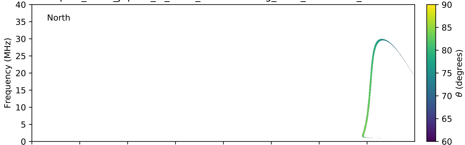
expres_earth_jupiter_io_isaac_lossc-wid1deg_3kev_20080103_v01.cdf
