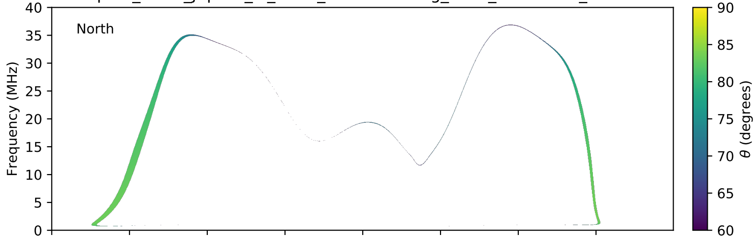
expres_earth_jupiter_io_isaac_lossc-wid1deg_3kev_20080102_v01.cdf
