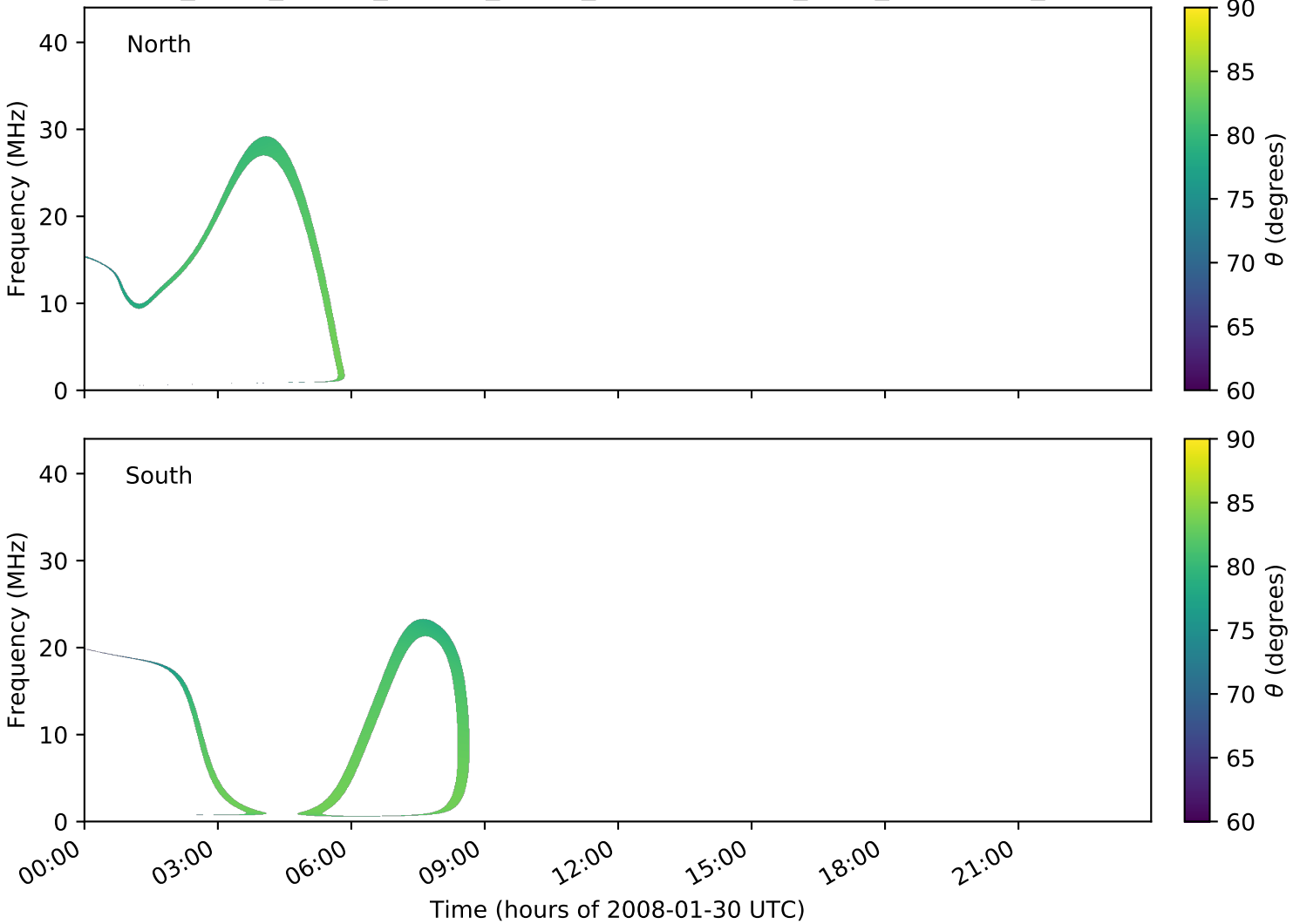
expres_earth_jupiter_europa_jrm09_lossc-wid1deg_3kev_20080130_v01.cdf
