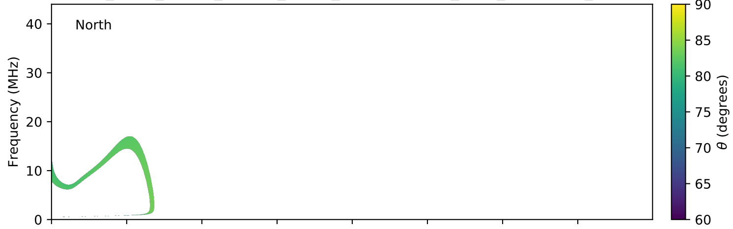
expres_earth_jupiter_europa_jrm09_lossc-wid1deg_3kev_20080123_v01.cdf
