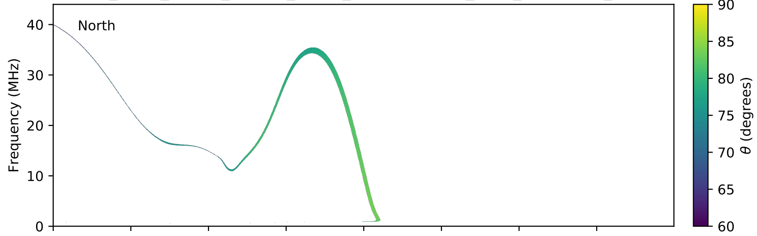
expres_earth_jupiter_europa_jrm09_lossc-wid1deg_3kev_20080119_v01.cdf
