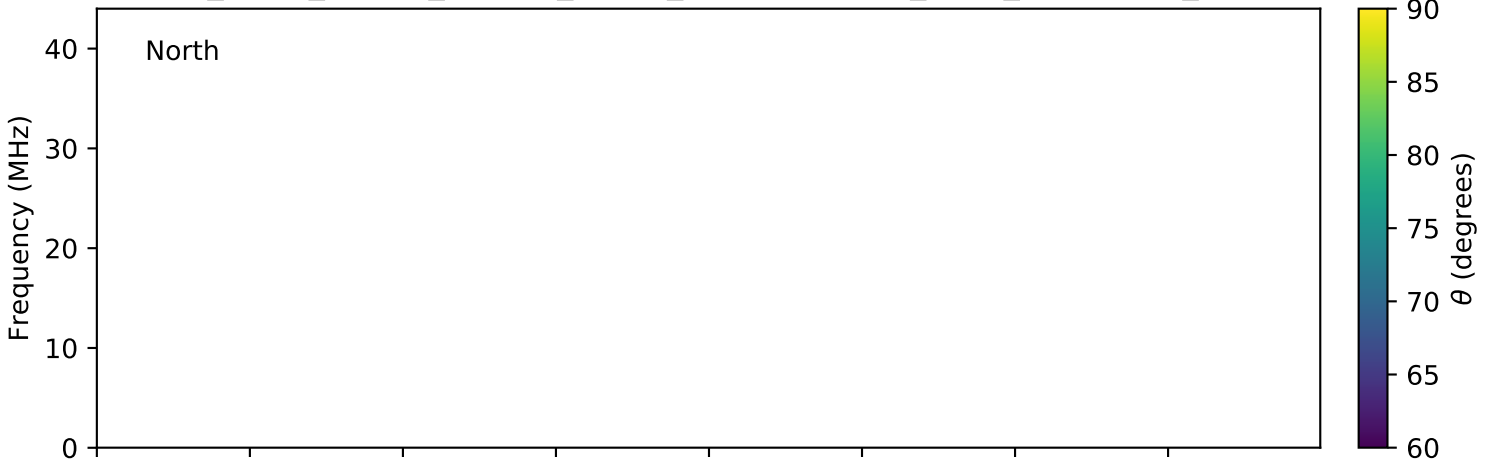
expres_earth_jupiter_europa_jrm09_lossc-wid1deg_3kev_20080109_v01.cdf
