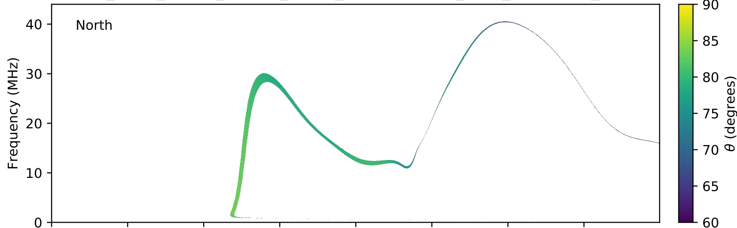
expres_earth_jupiter_europa_jrm09_lossc-wid1deg_3kev_20080107_v01.cdf
