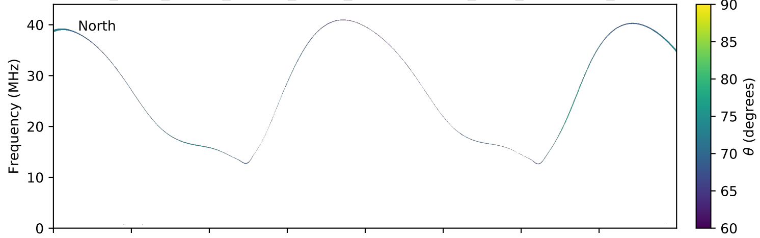
expres_earth_jupiter_europa_jrm09_lossc-wid1deg_3kev_20080104_v01.cdf
