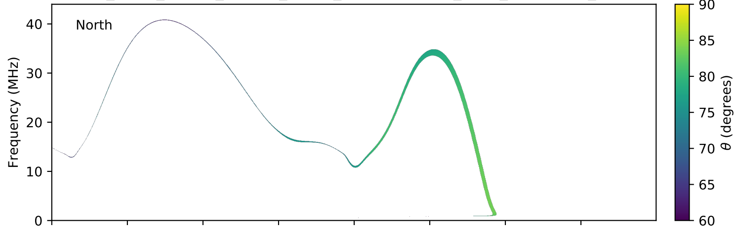
expres_earth_jupiter_europa_jrm09_lossc-wid1deg_3kev_20080101_v01.cdf
