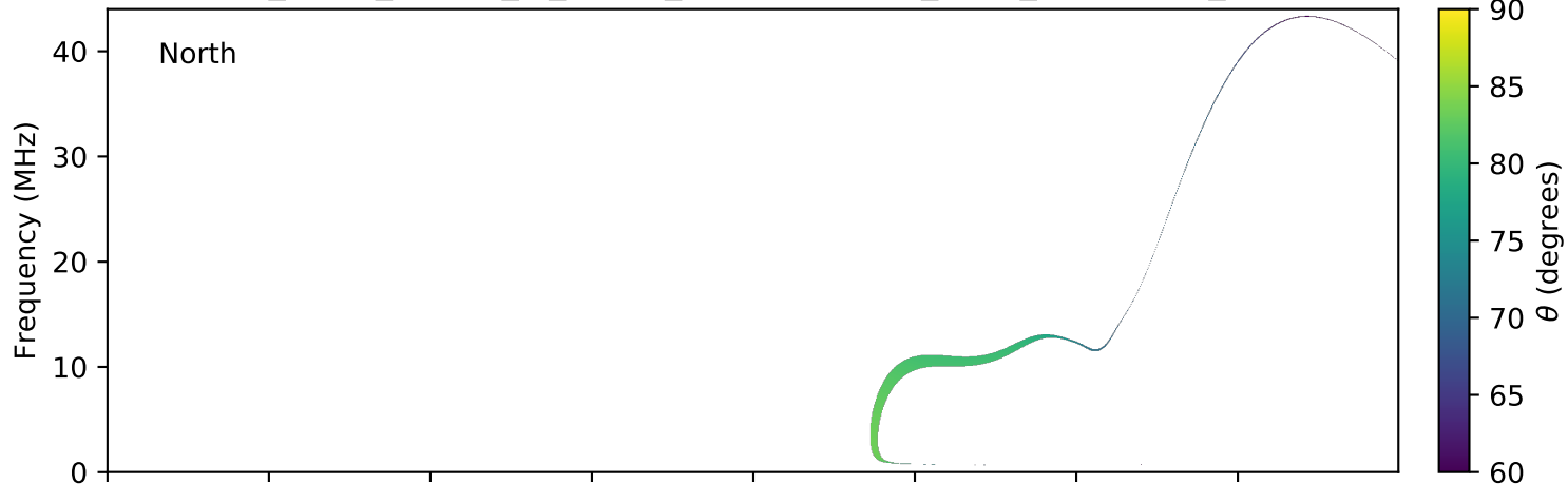
expres_earth_jupiter_io_jrm09_lossc-wid1deg_3kev_20071213_v01.cdf
