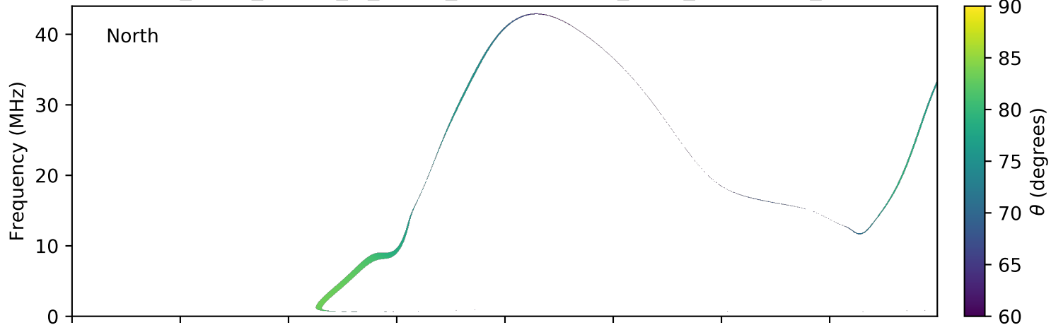
expres_earth_jupiter_io_jrm09_lossc-wid1deg_3kev_20071208_v01.cdf
