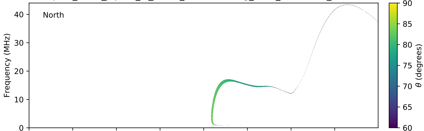
expres_earth_jupiter_io_jrm09_lossc-wid1deg_3kev_20071206_v01.cdf
