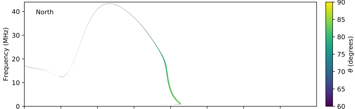
expres_earth_jupiter_io_jrm09_lossc-wid1deg_3kev_20071205_v01.cdf
