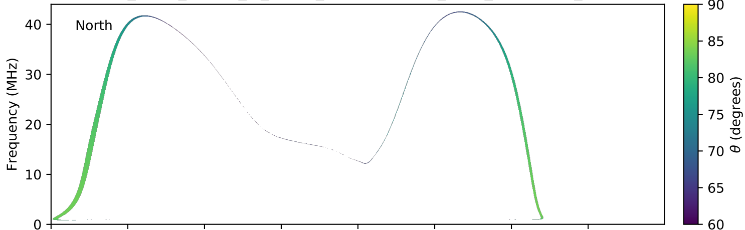
expres_earth_jupiter_io_jrm09_lossc-wid1deg_3kev_20071203_v01.cdf
