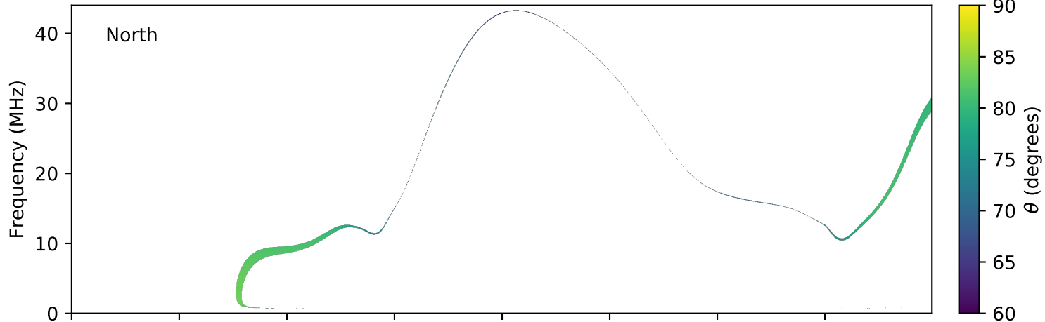
expres_earth_jupiter_io_jrm09_lossc-wid1deg_3kev_20071201_v01.cdf
